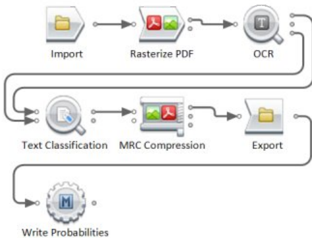
Illustration 5: DocYard-Workflow
