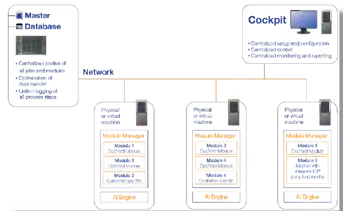
Illustration 3: DocYard Architecture
