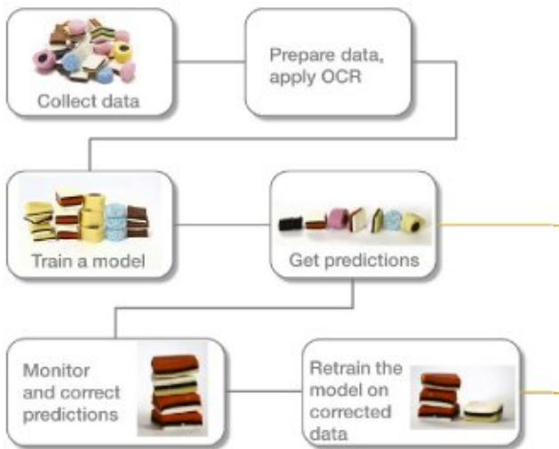
Illustration 1: Typical Workflow
